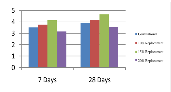
CHART 2: SPLIT TENSILE STRENGTH
